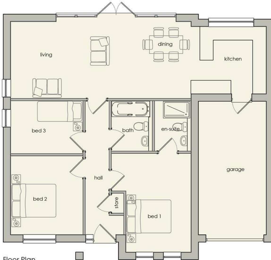
Floor Plan
